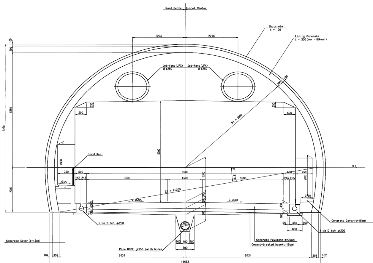
Fig 1: Typical Cross- section of Main Tunnel (all dimensions are in mm)
