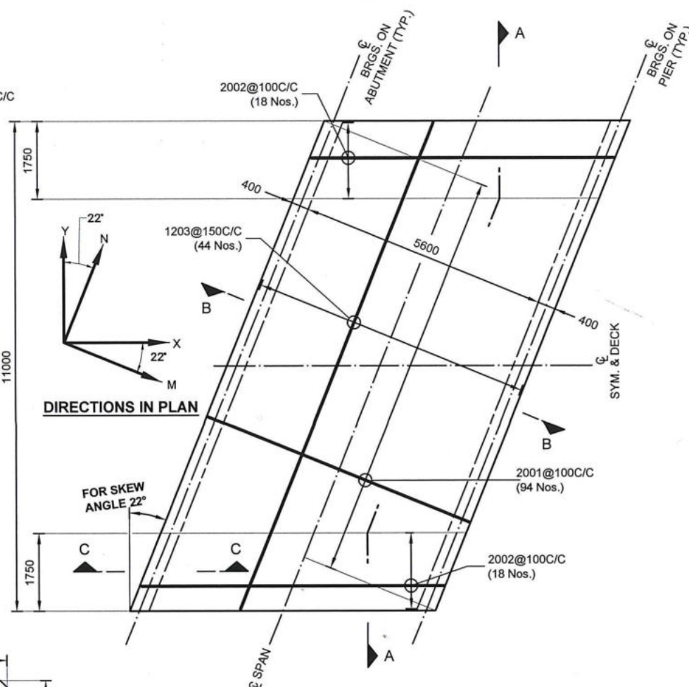
PLAN SHOWING ONLY BOTTOM REINFORCEMENT DETAILS OF SLAB DECK
