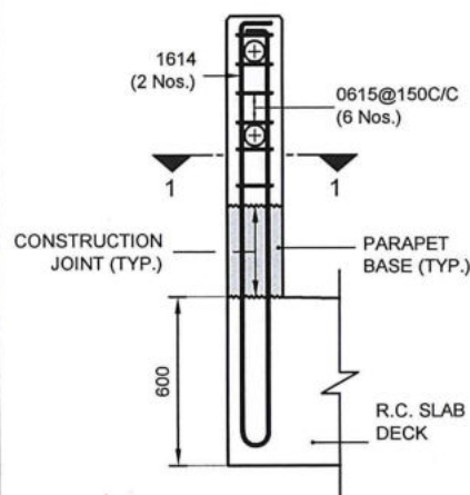
PARAPET POST DETAIL
