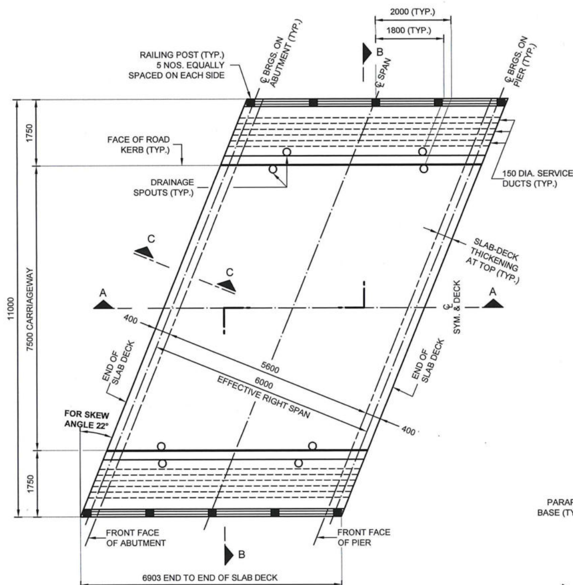
PLAN (APPROACH SLAB NOT SHOWN)
