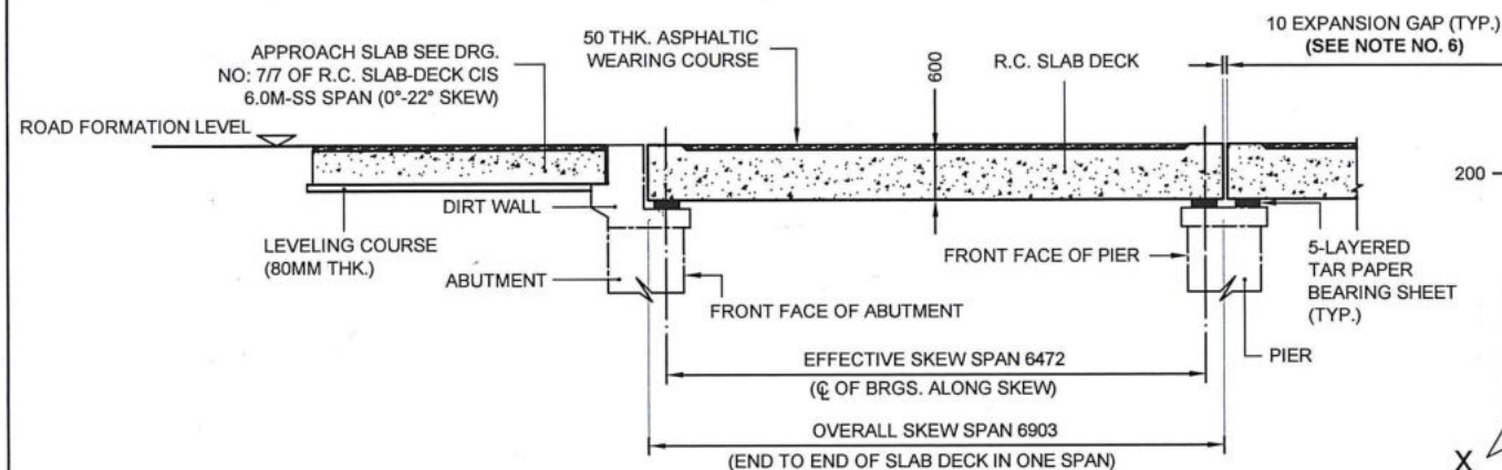
SECTION A-A (ROAD KERBS & PARAPET RAILINGS NOT SHOWN)
