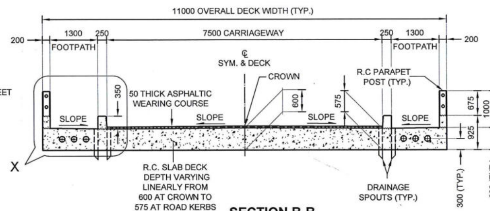
SECTION B-B
