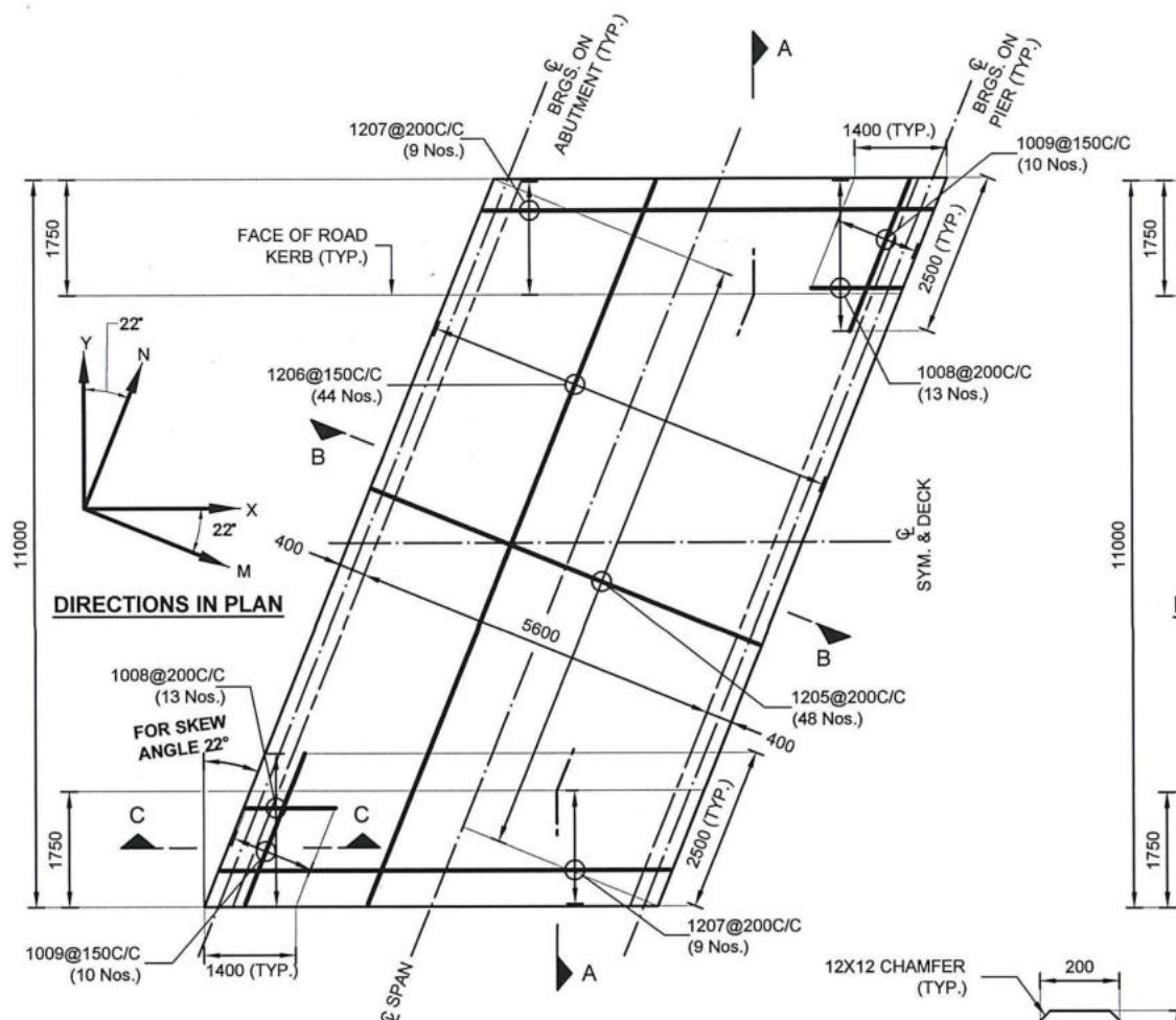
PLAN SHOWING ONLY TOP REINFORCEMENT DETAILS OF SLAB DECK
