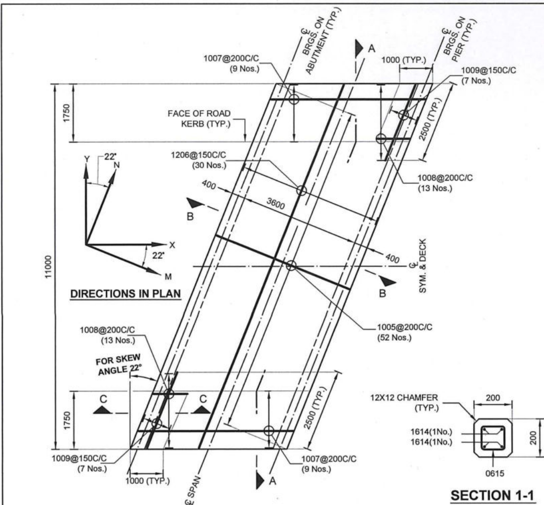
PLAN SHOWING ONLY TOP REINFORCEMENT DETAILS OF SLAB DECK (SERVICE DUCTS, ROAD KERBS AND PARAPET BASES NOT SHOWN)
