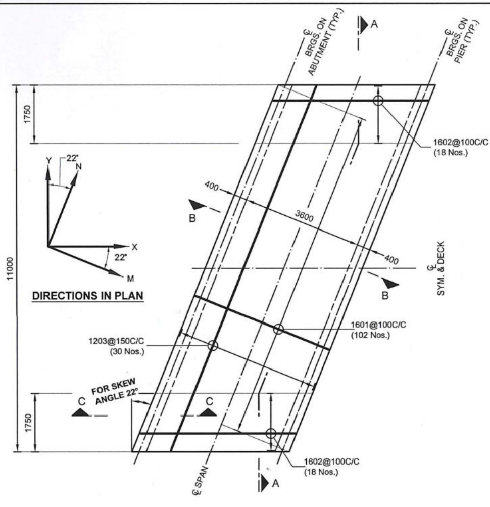
PLAN SHOWING ONLY BOTTOM REINFORCEMENT DETAILS OF SLAB DECK
