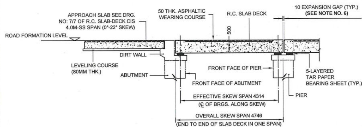
SECTION A-A (ROAD KERBS & PARAPET RAILINGS NOT SHOWN)
