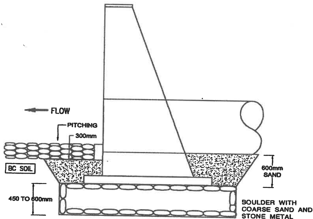
Fig. 22.1 Hume Pipe Culvert in BC Soil
