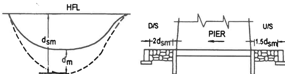
Fig. 21.1 Scour Depth and Apron Width for Raft
