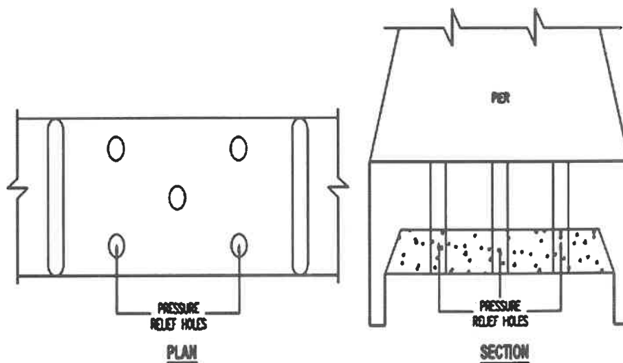
PRESSURE RELIEF HOLES IN RAFT SLAB
