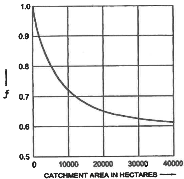
Fig. 4.2 'f' curve
