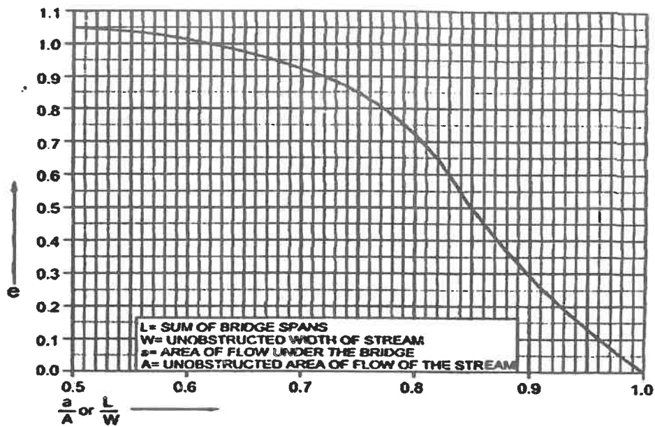
Fig. 15.3 Elements of the hydraulics of flow through bridges The orifice formula coefficient " e "
