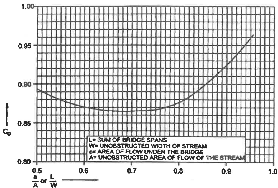
Fig. 15.4 The Orifice Formula Coefficient " C_Q "
