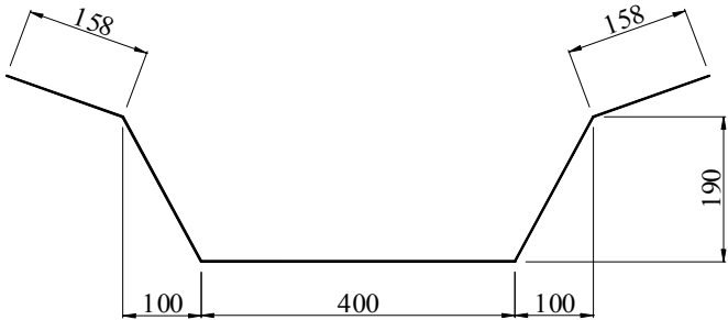
VALLEY GUTTER
