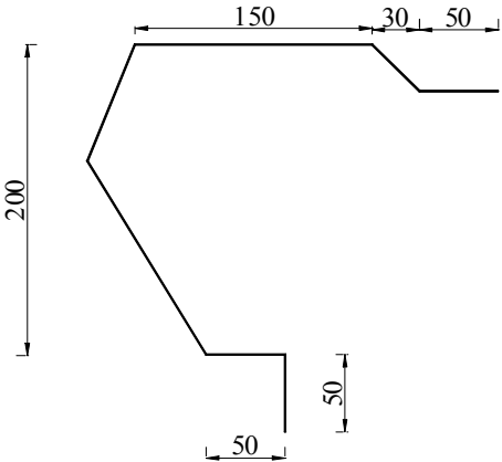
EAVE & PEAK FASCIA
