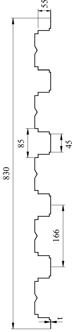
PROFILE OF STEEL DECKING
