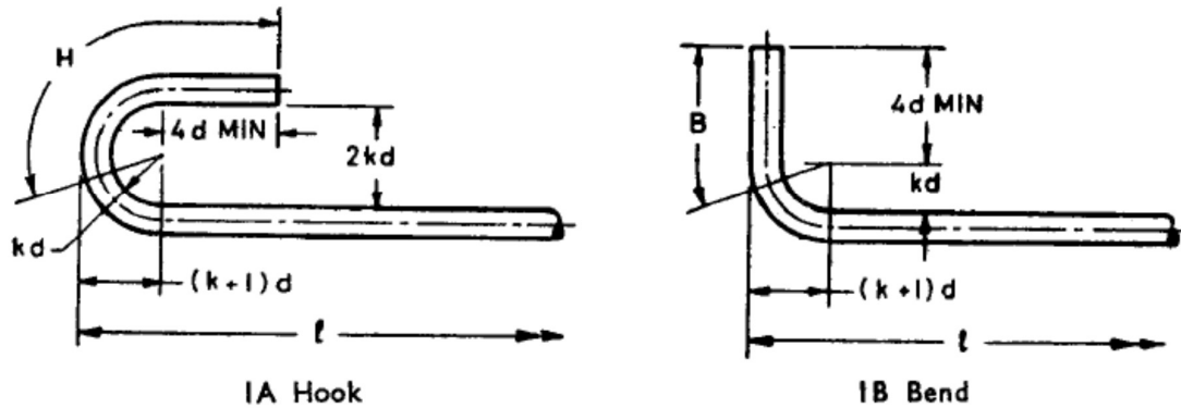
Figure 2.1 : Hook and Bend Details
