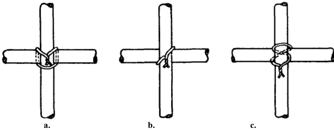
Figure 2.2 Three methods of tying reinforcement bars
