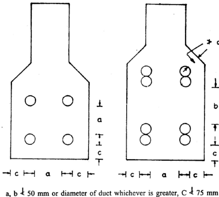
Figure 2.3 Cable Cover
