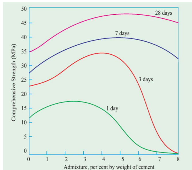
Figure 1.2 : Effect of Admixture Dose
