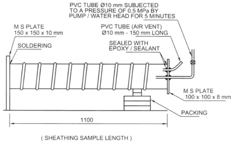
Figure 1.4 Test For Water Loss Study
