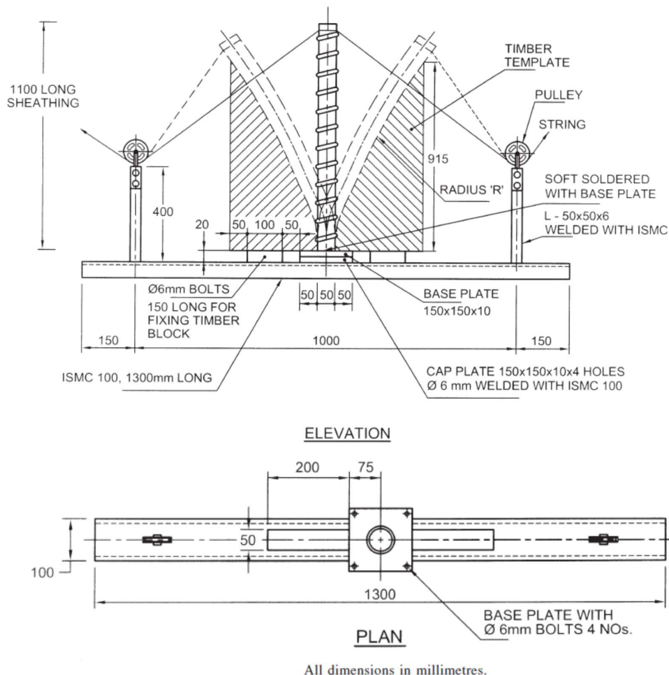
Figure 1.2 Workability Test
