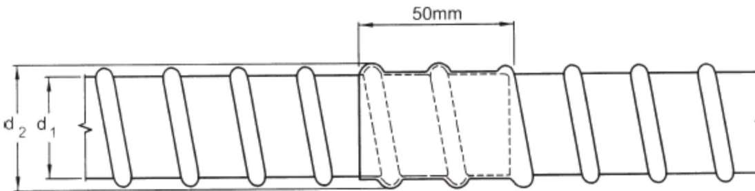
Figure 1.6 Typical details heat-shrink coupler
