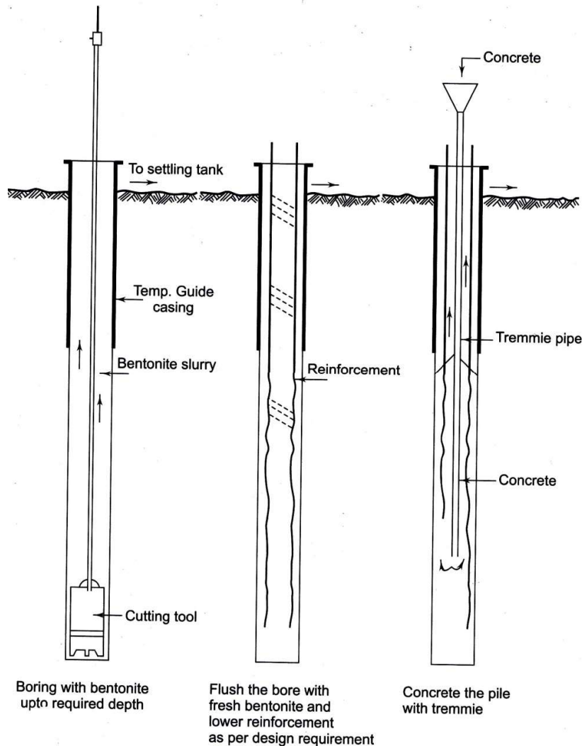
Figure 3.b Schematic drawing of concreting in Bored Pile
