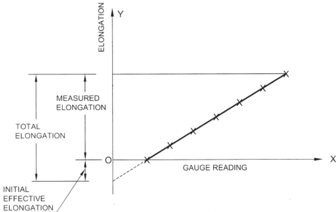
Figure 4.1 Determination of Actual Elongation
