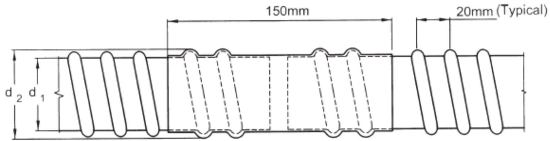
Figure 1.5 Typical details of a sleeve coupler
