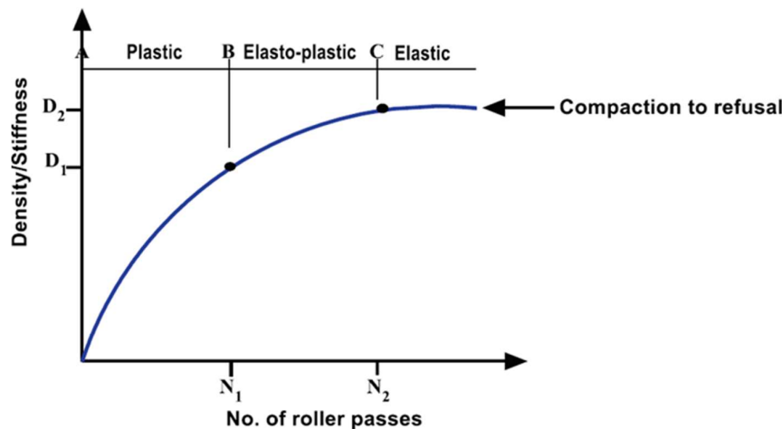
Figure 3-7: Illustration of concept of compaction to refusal
