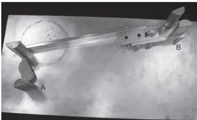
Figure 2.2 Measuring Flat and Elongated Particles
