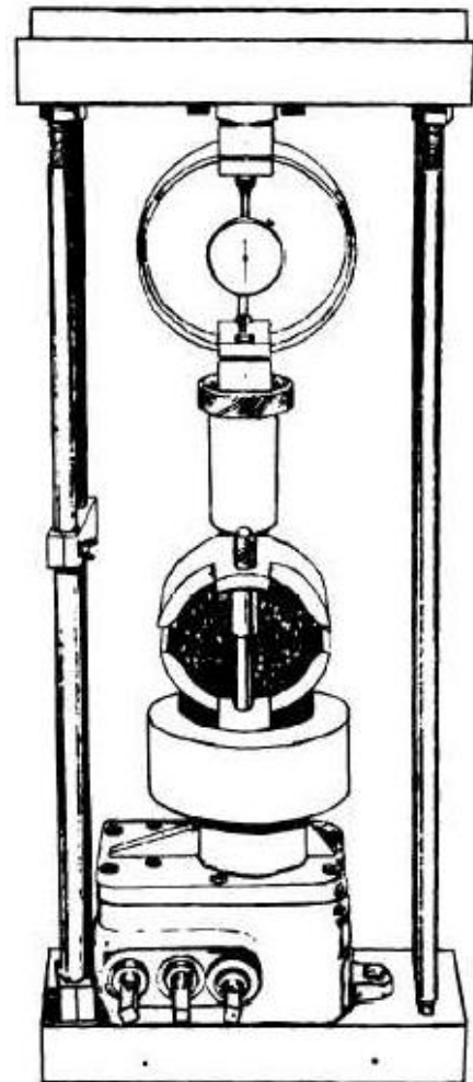
Figure 3.8 Marshall Apparatus
