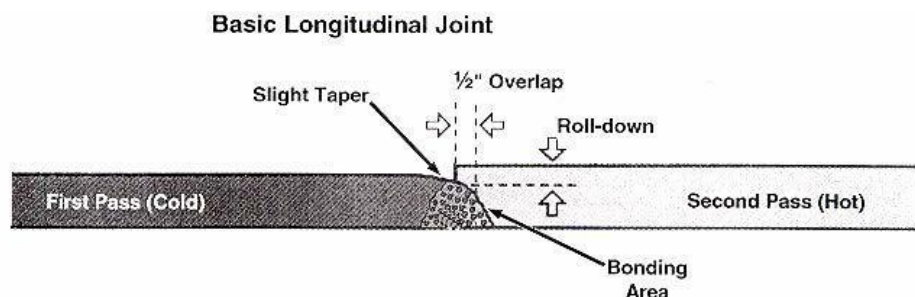
Figure 5.6 Traditional “butt” joint
