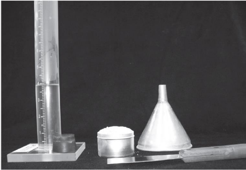
Figure 2.3 Sand Equivalent Test
