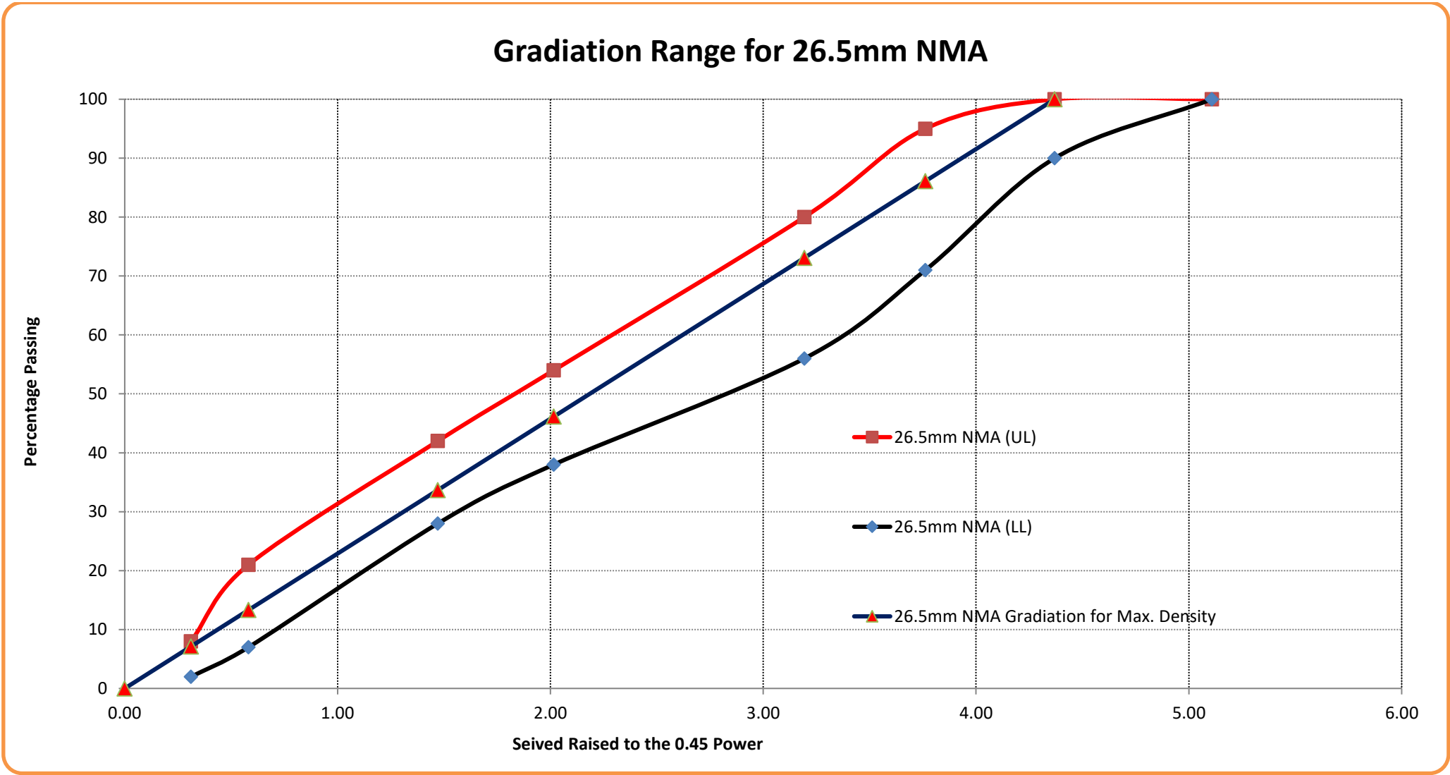
Figure 2.6 : Maximum Density line and Upper-Lower Limit of Gradation as per specification in 0.45 Power Chart (26.5mm NMAS )
