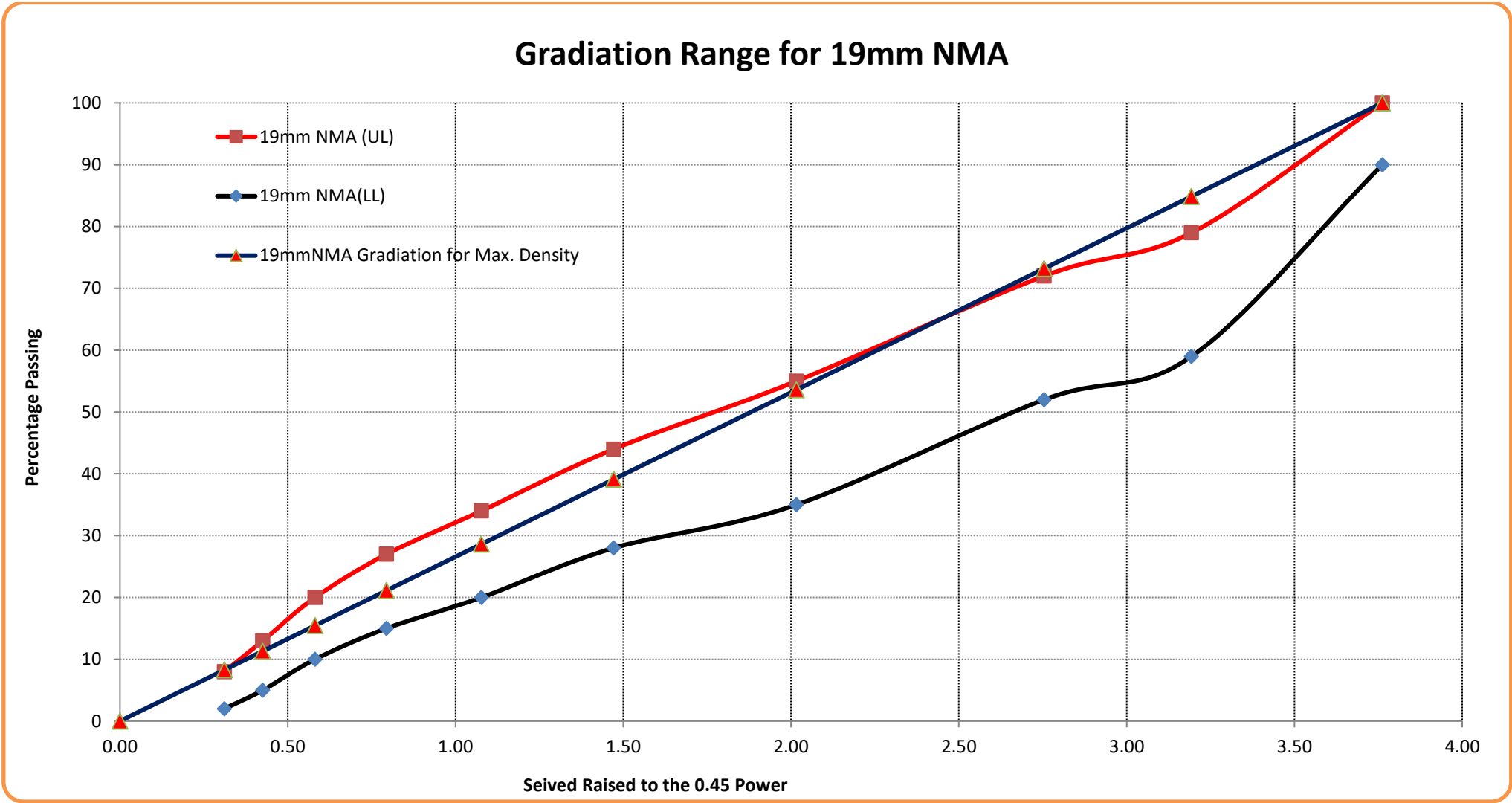
Figure 2.5 : Maximum Density line and Upper-Lower Limit of Gradation as per specification in 0.45 Power Chart (19 mm NMAS )
