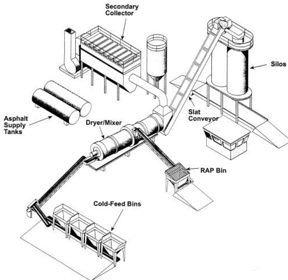
Figure 4.5 Major plant components of parallel-flow drum-mix plant
