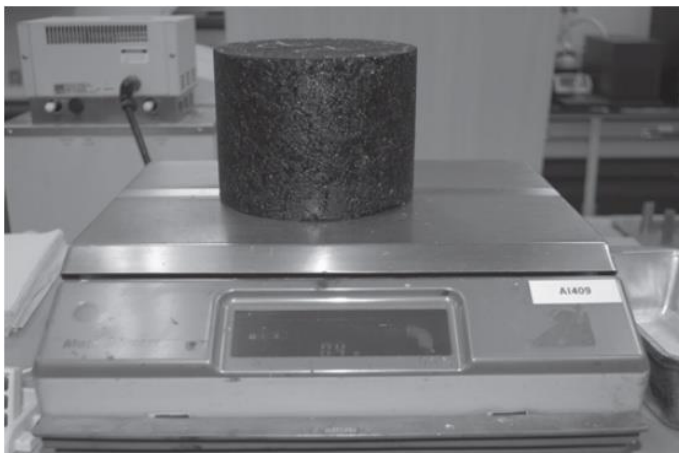
Figure 3.6 Determination of dry mass of specimen
