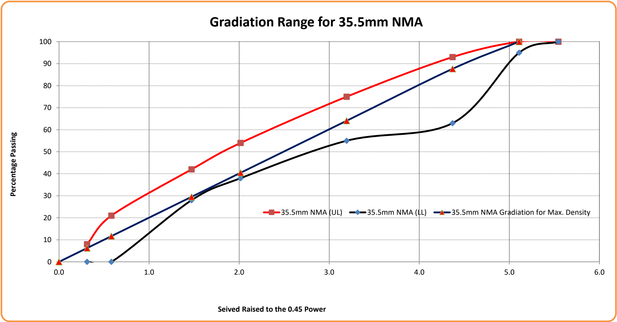
Figure 2.7 : Maximum Density line and Upper-Lower Limit of Gradation as per specification in 0.45 Power Chart (35.5mm NMAS )
