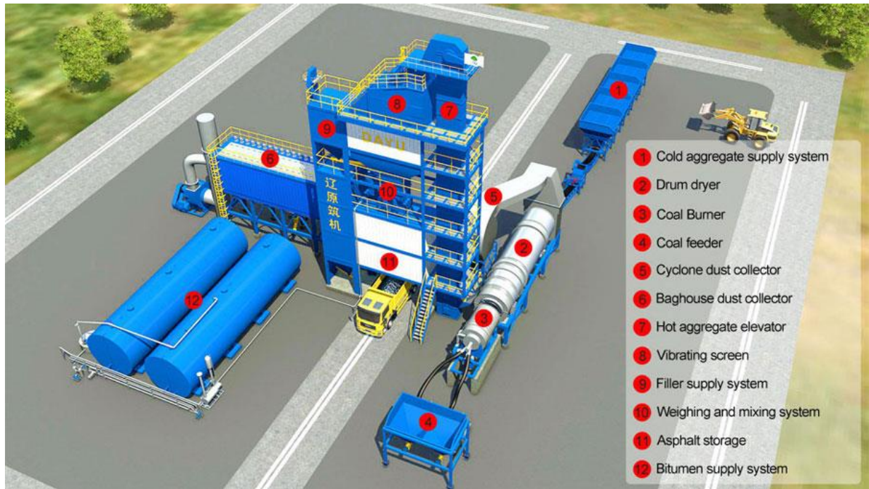
Figure 4.2 Major components of Batch Plant
