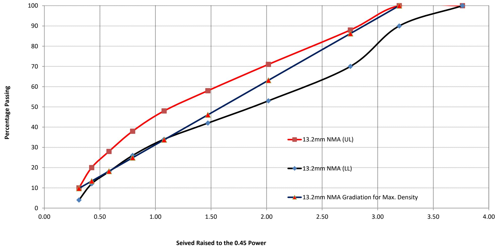
Figure 2.4 : Maximum Density line and Upper-Lower Limit of Gradation as per specification in 0.45 Power Chart (13.2mm NMAS )
