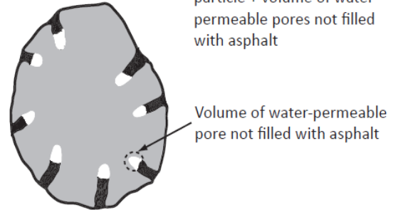
Figure 3.8 Illustration of Effective Aggregate
