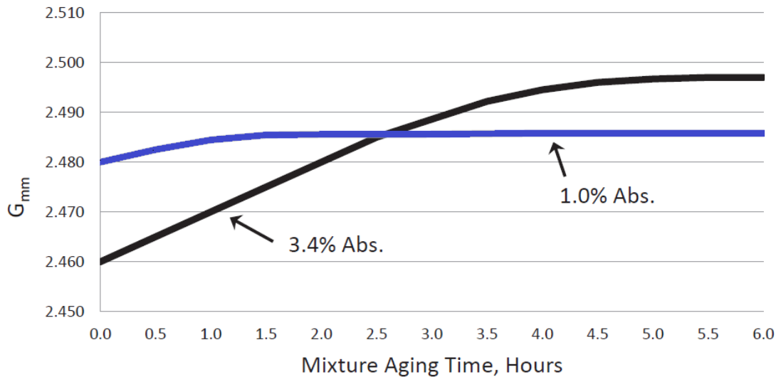
Figure 3.4 Effects of absorption on G_{mm}
