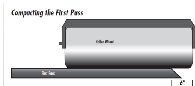
Figure A3.1 Unsupported edge compaction
