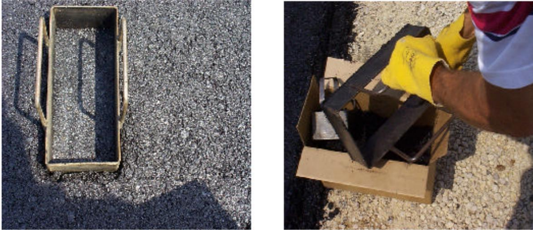
Figure 6.1 Template Placed in Asphalt Mat Cleaning Asphalt Off Template into Sample Container
