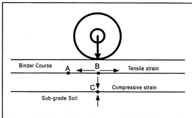
Figure 3: Critical Locations on Pavement
