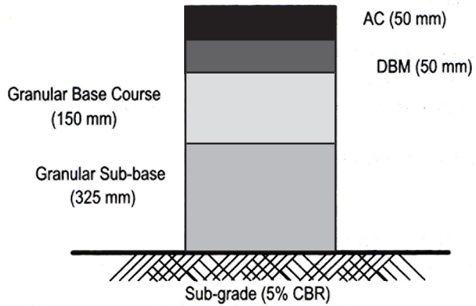
Figure 2: Cross section of the designed pavement
