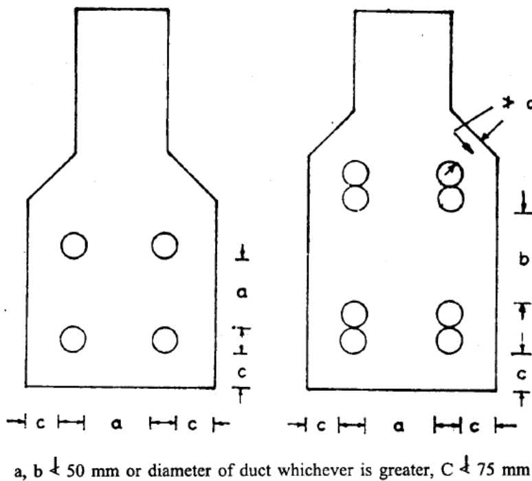
Figure 2.3 Cable Cover
