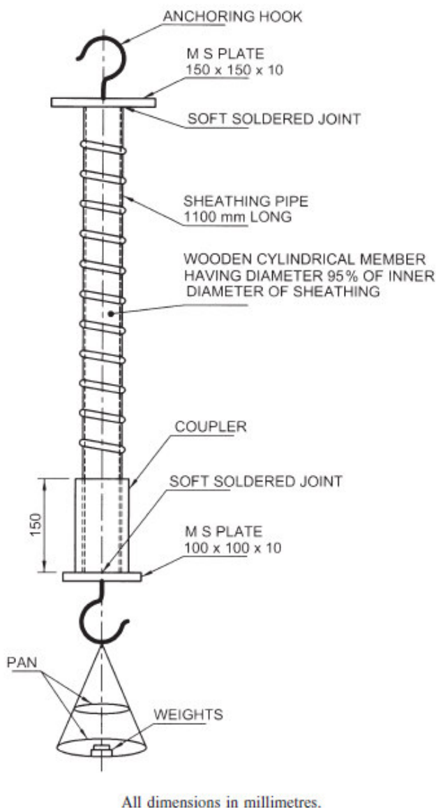
Figure 1.3 Tension Load Test
