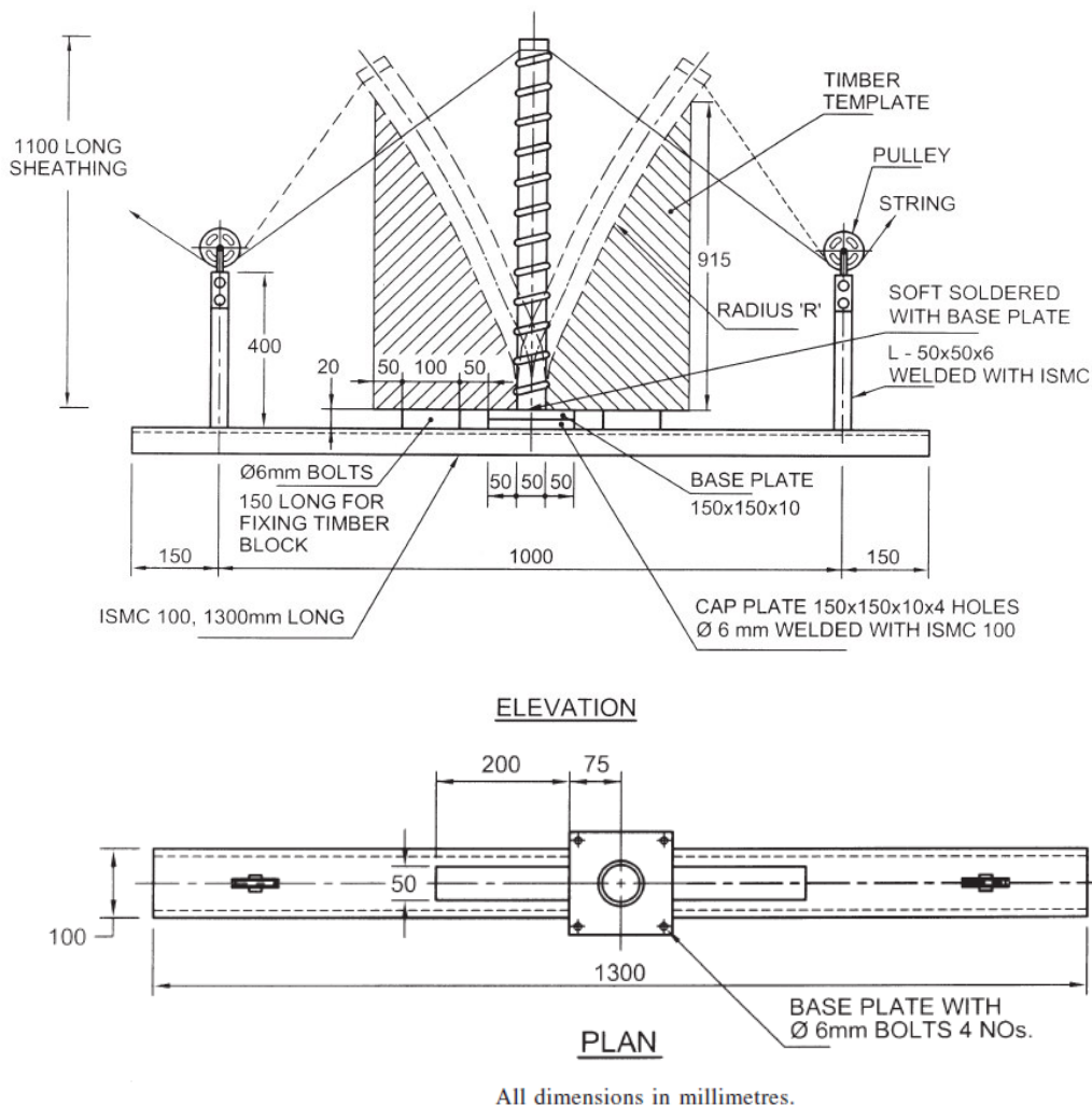
Figure 1.2 Workability Test
