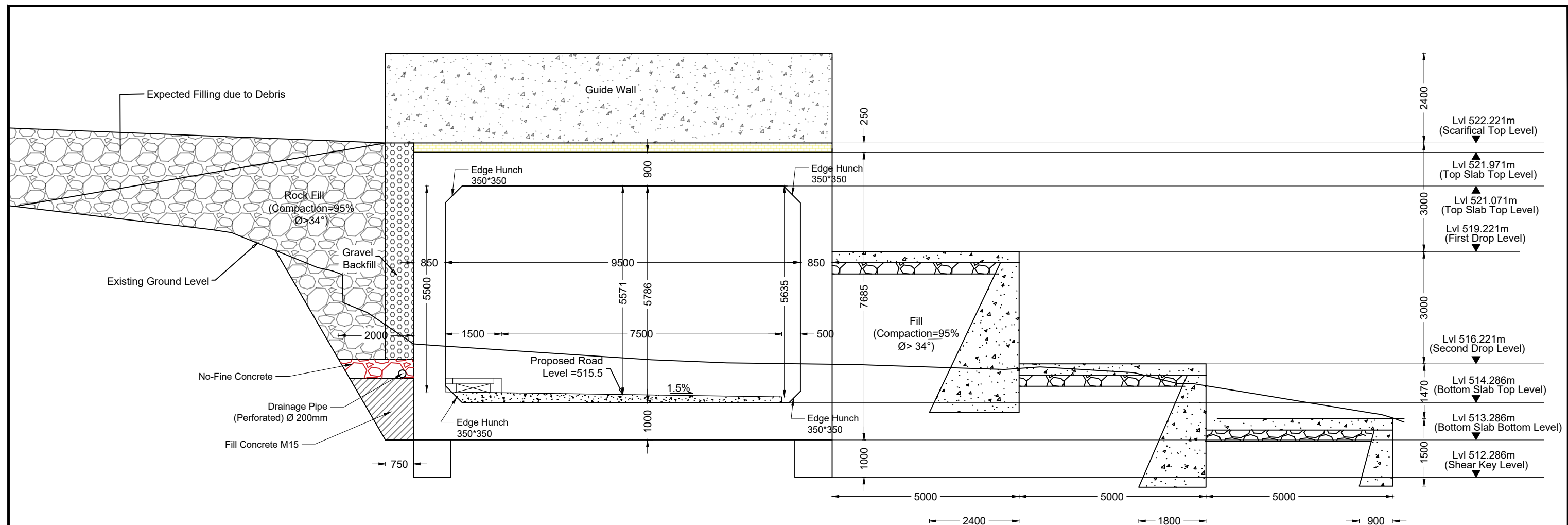
FRONT ELEVATION VIEW OF GALLERY
