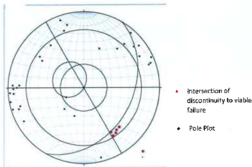
Figure 7: Stereographic projection of major discontinuities measured at chainage 591+300 for slope stability analysis
