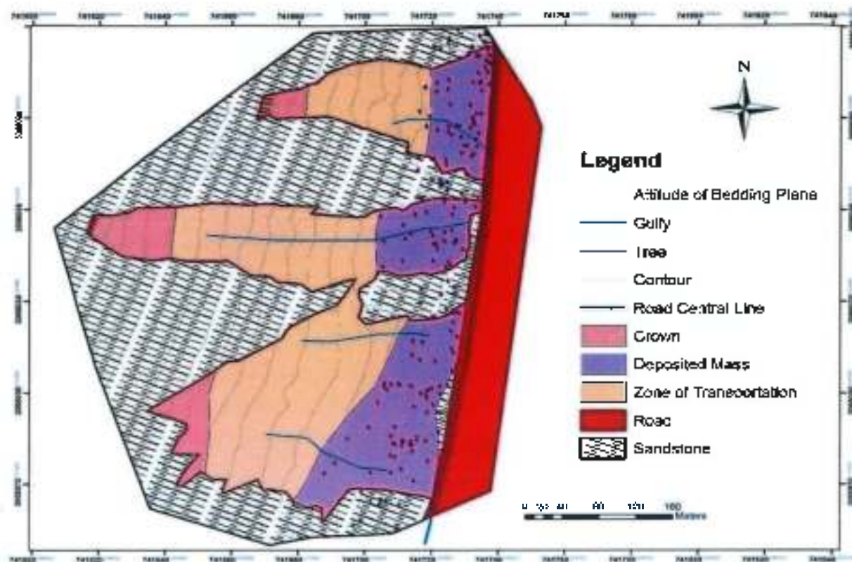
Figure 2: Geomorphology and Geological Map around Landslide area
